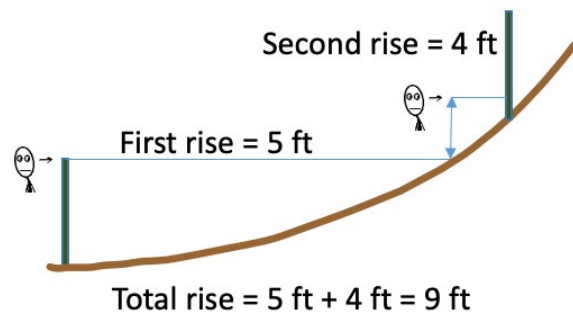
Figure 10b. The stakes are 5 feet tall. The first level line hits the ground in front of the uphill stake, where the student kneels or stands and projects a second level line. The second level line hits 4 feet below the top of the uphill stake. Eyesight image courtesy of clipartfest.com . Drawing by John M. Galbraith, Virginia Tech.
